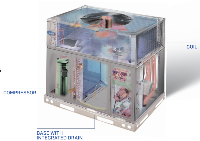
PACKAGED GAS FURNACE/AIR CONDITIONER SHOWN
